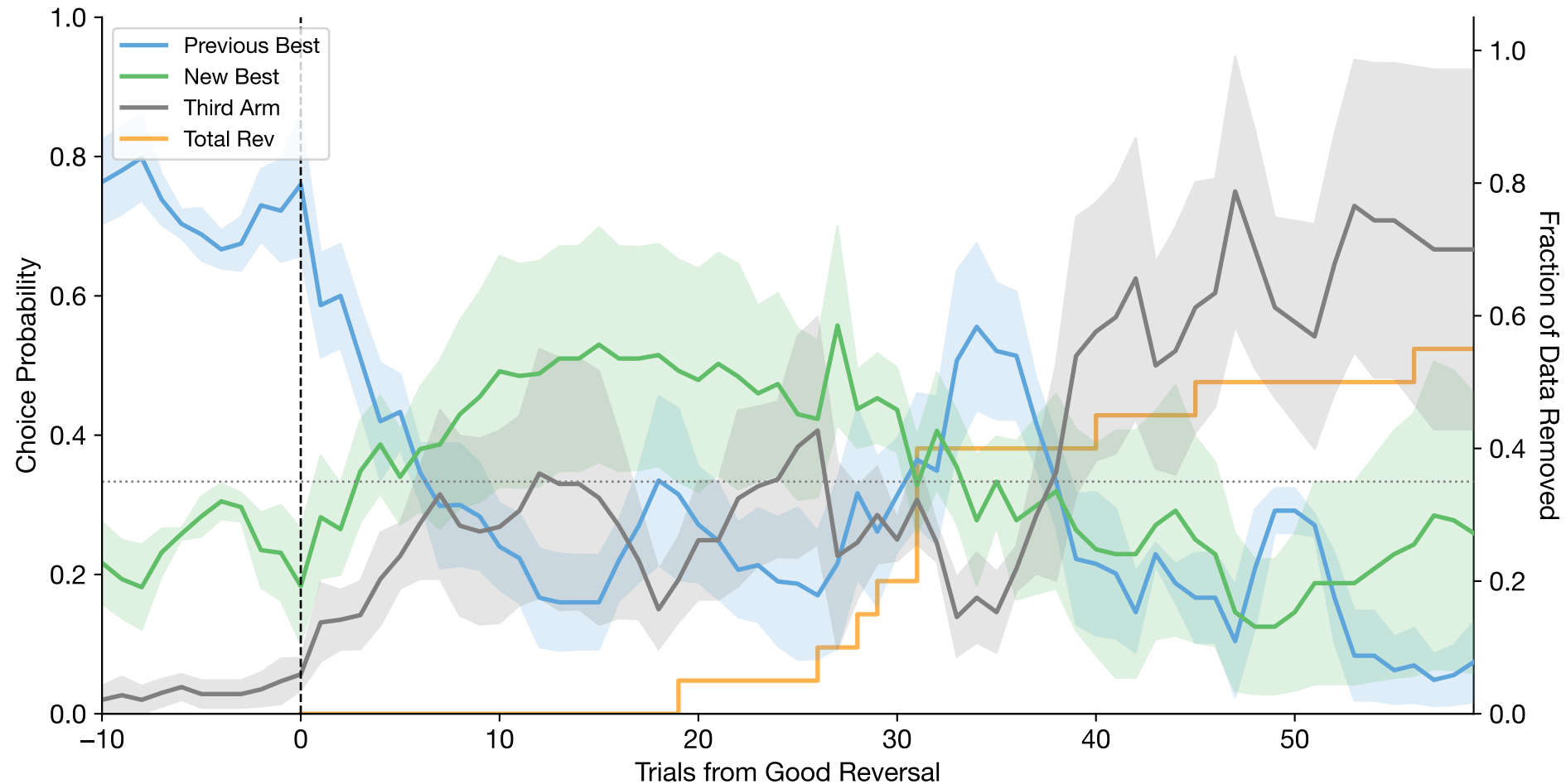
Good Reversal-Aligned Choices (mean \pm se across subjects | n=5 subjects, n=20 reversals)
